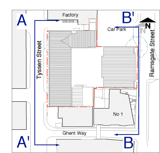
Key Plan 1:1000
